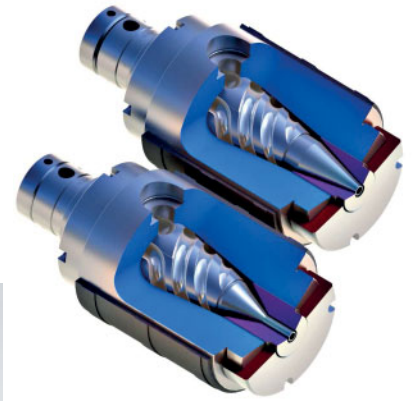
Photos of The Bullet II, showing the absence of hardware, i.e. nuts and bolts, so disassembly, cleaning and restart are made easier
