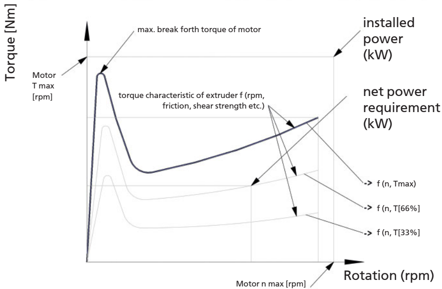
Efficiency curve of a motor (Source: Kabel.Consult.Ing)
