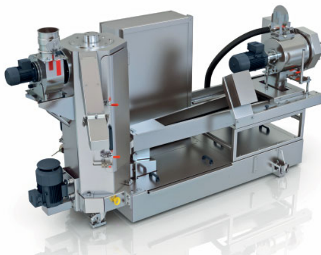
BKG® WRP 1000 Water Ring Pelletizer
